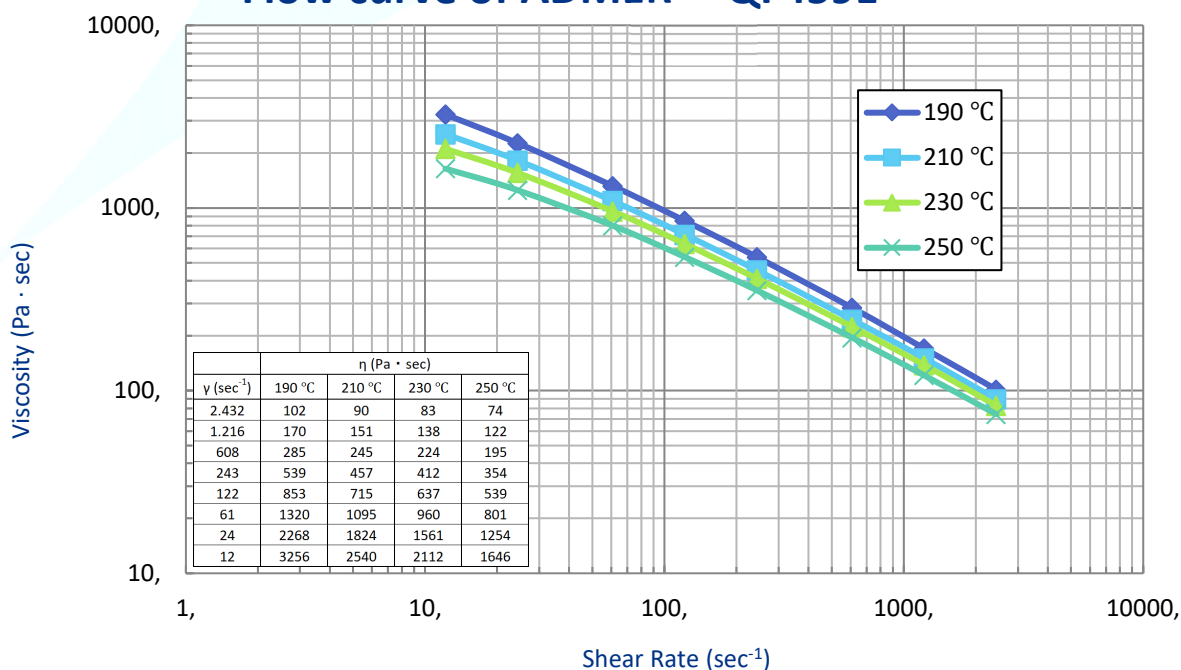
Flow curve of ADMER™ QF459E
