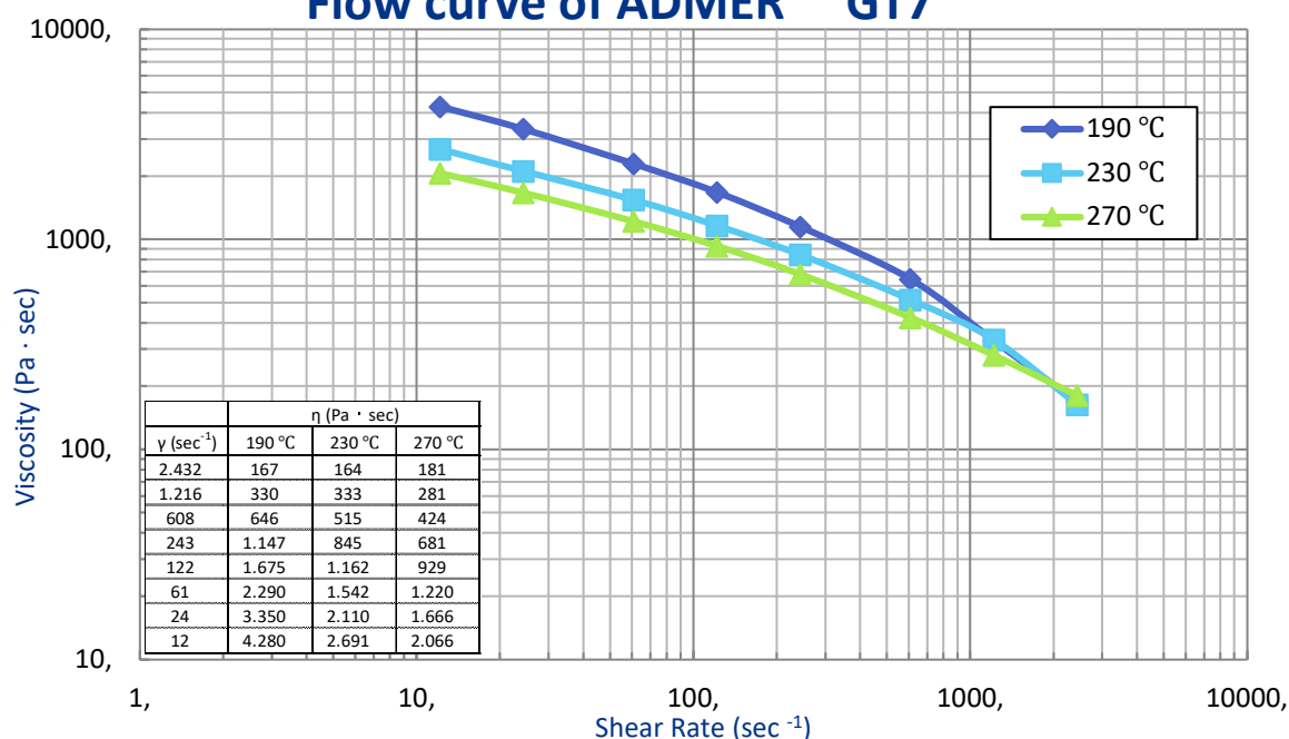
Flow curve of ADMER™ GT7
