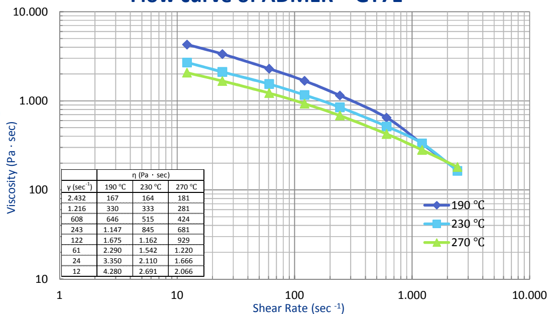
Flow curve of ADMER™ GT7E
