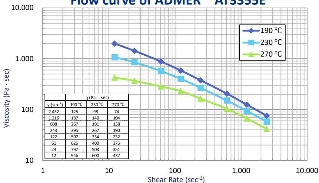
Flow curve of ADMER™ AT3355E
